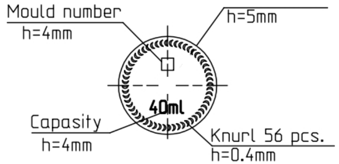
View A
